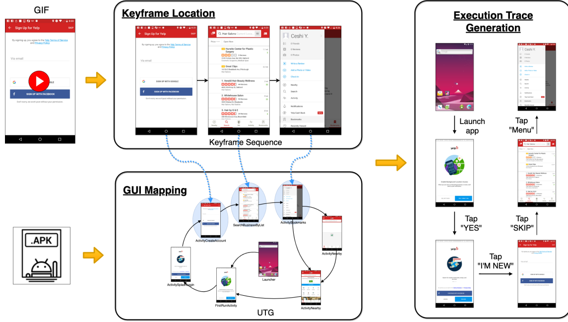
Figure 1: The overview of GIFdroid.
