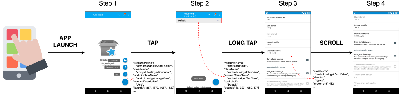
Figure 2: Example of execution trace generated by GIFdroid.
